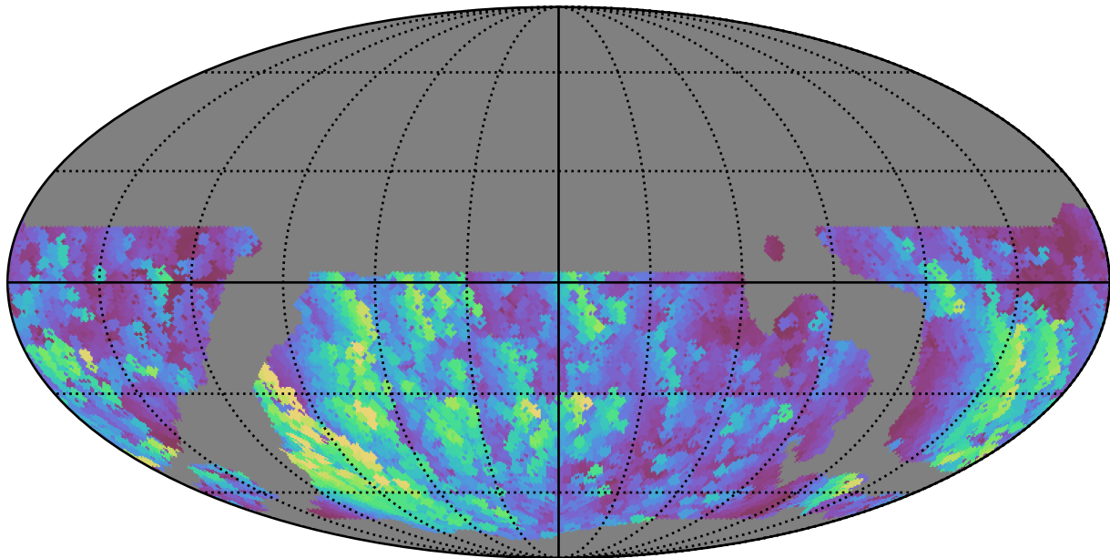
weather_cloudso4v3.4_10yrs WFD u band: Max normairmass
