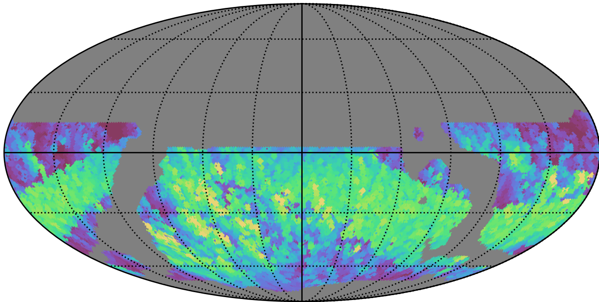
weather_cloudso4v3.4_10yrs WFD r band: Max normairmass
