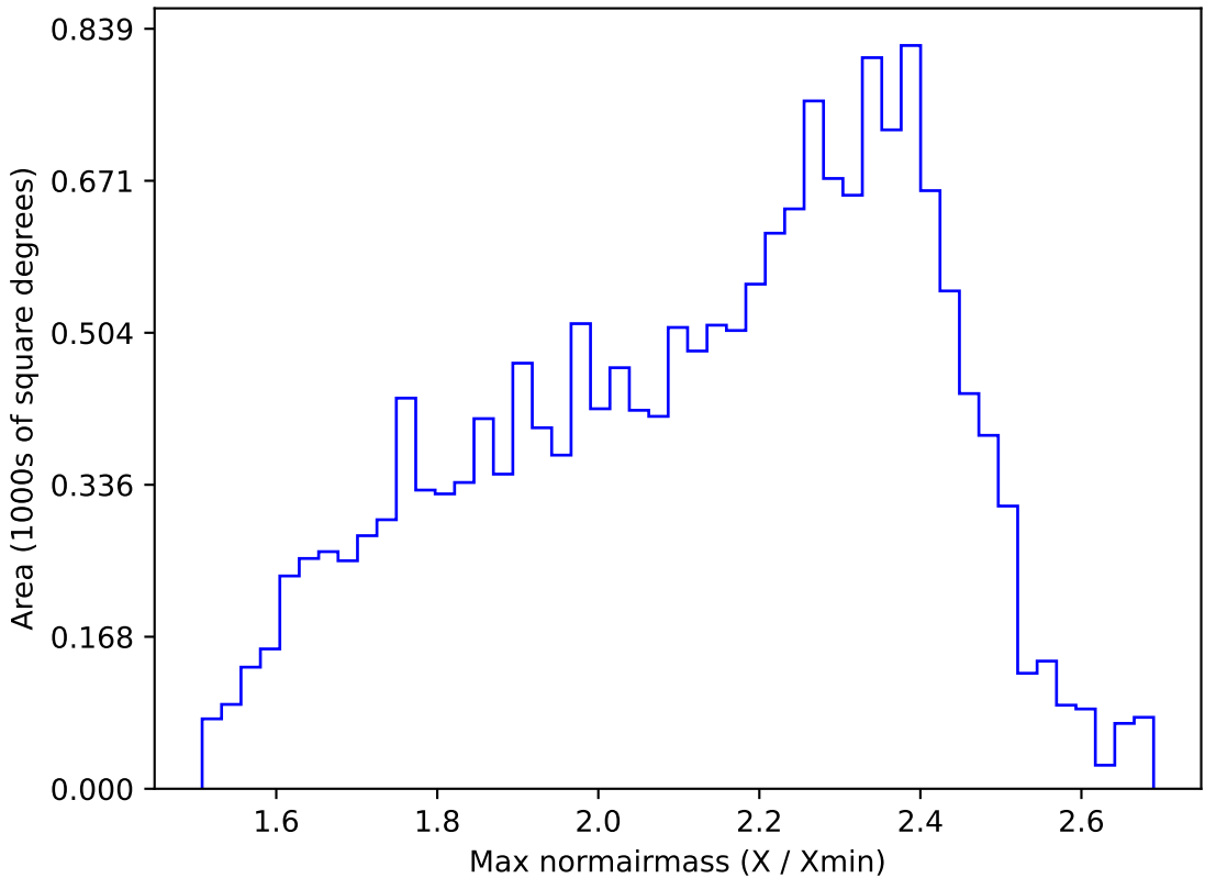
weather_cloudso4v3.4_10yrs WFD r band: Max normairmass
