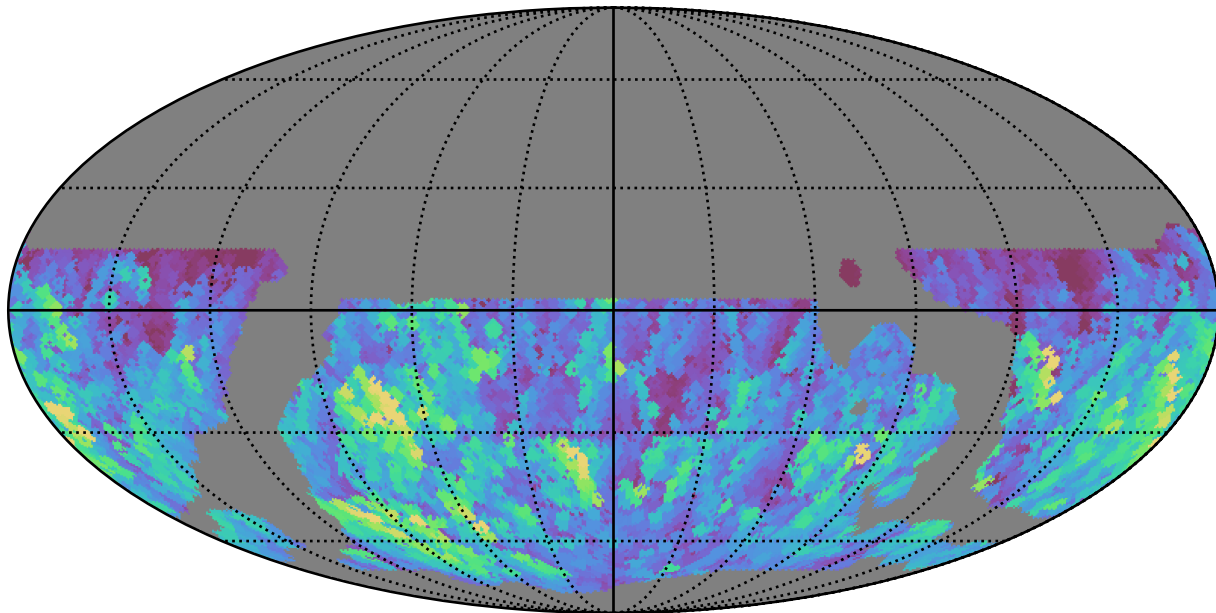
weather_cloudso4v3.4_10yrs WFD g band: Max normairmass
