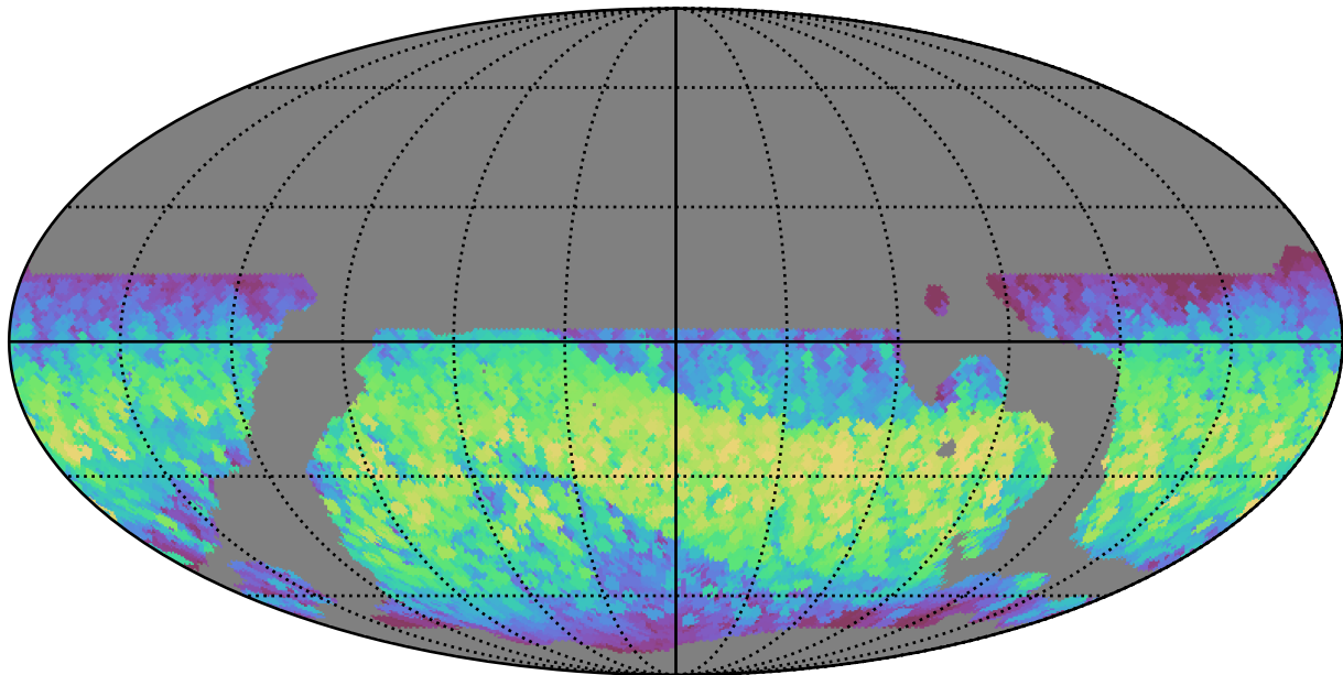
weather_cloudso4v3.4_10yrs WFD all bands: Max normairmass
