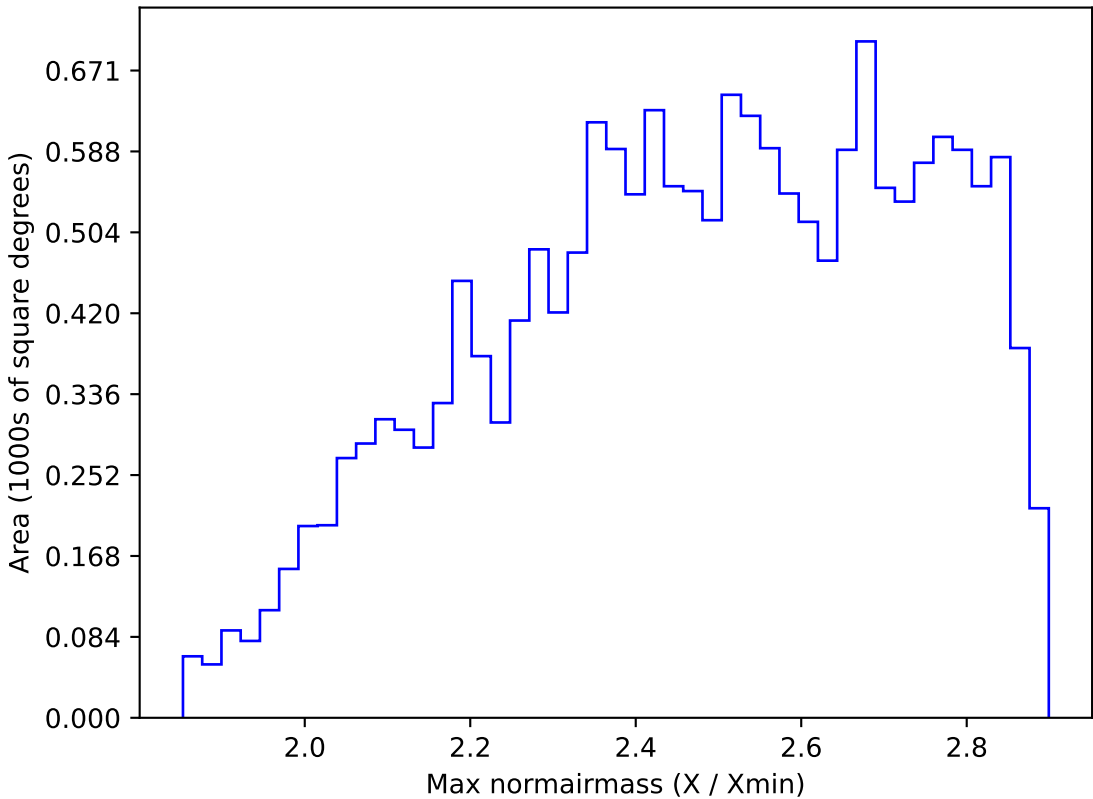
weather_cloudso4v3.4_10yrs WFD all bands: Max normairmass
