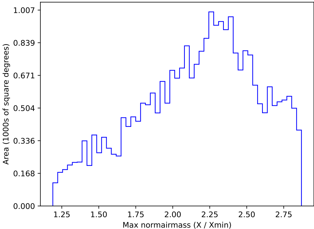
weather_cloudso4v3.4_10yrs All sky z band: Max normairmass
