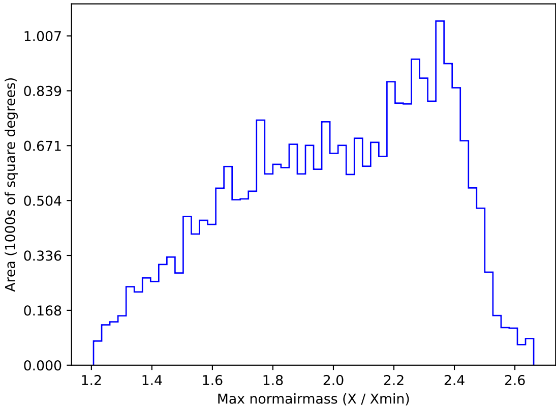
weather_cloudso4v3.4_10yrs All sky r band: Max normairmass
