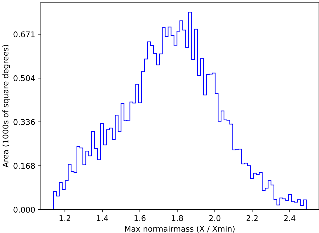
weather_cloudso4v3.4_10yrs All sky g band: Max normairmass
