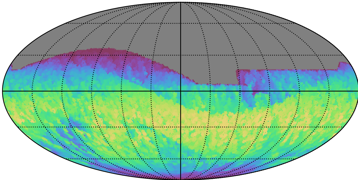
weather_cloudso4v3.4_10yrs All sky all bands: Max normairmass
