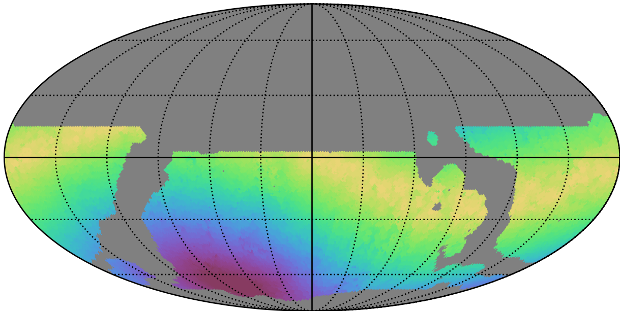
weather_cloudso4v3.4_10yrs WFD z band: Max moonDistance
