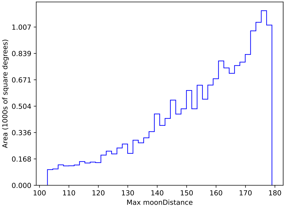
weather_cloudso4v3.4_10yrs WFD z band: Max moonDistance
