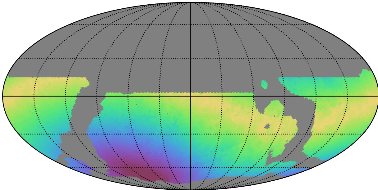
weather_cloudso4v3.4_10yrs WFD u band: Max moonDistance
