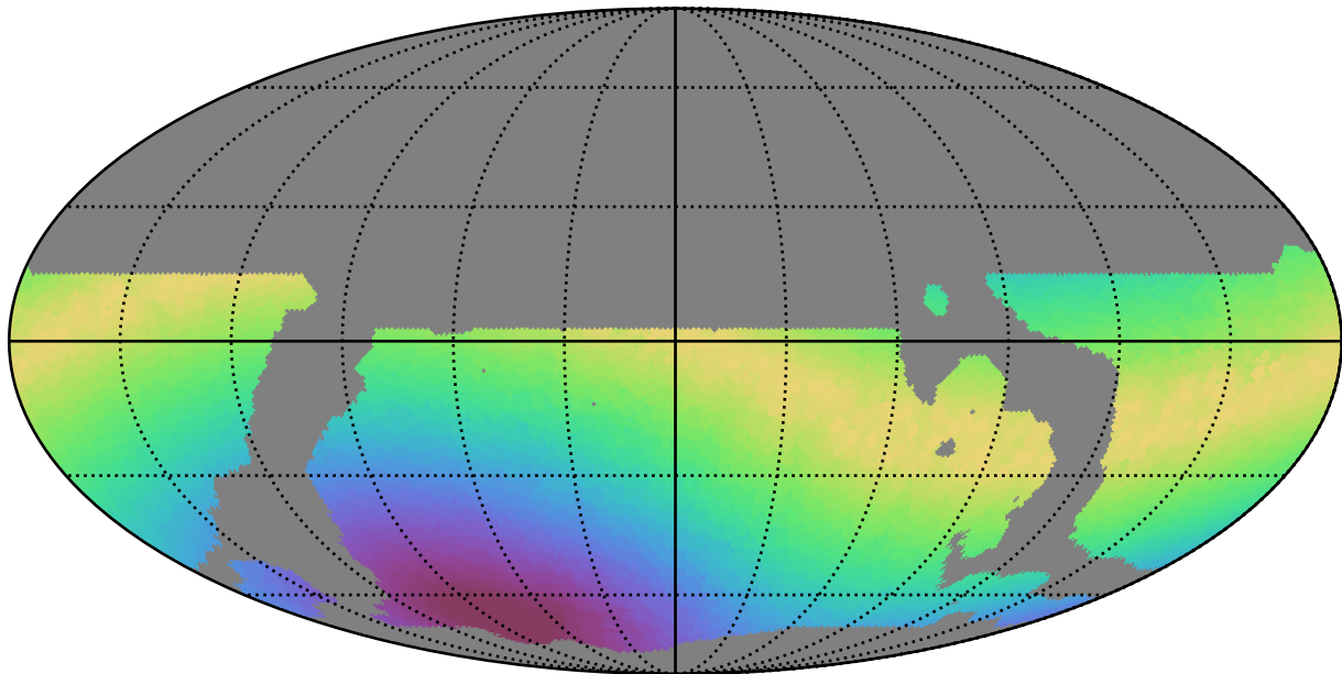
weather_cloudso4v3.4_10yrs WFD r band: Max moonDistance
