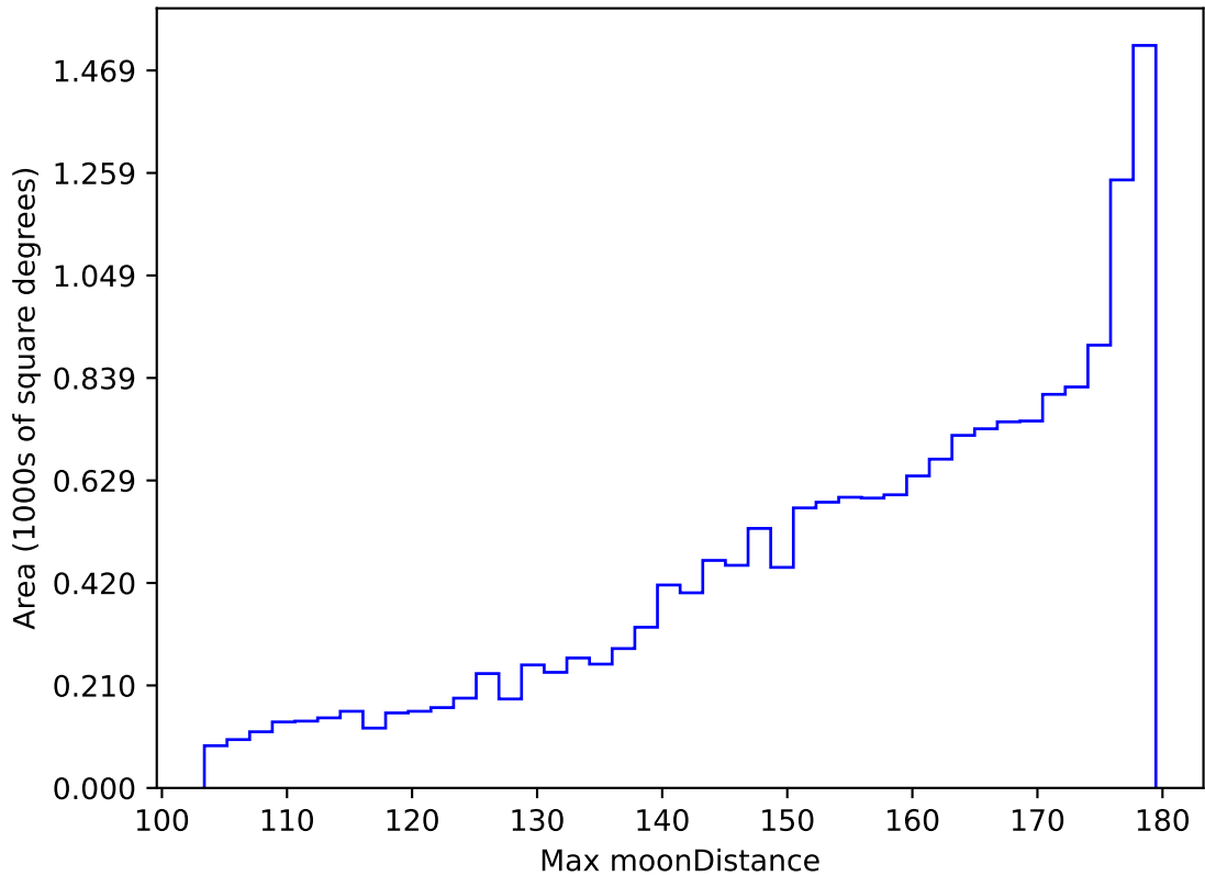
weather_cloudso4v3.4_10yrs WFD r band: Max moonDistance
