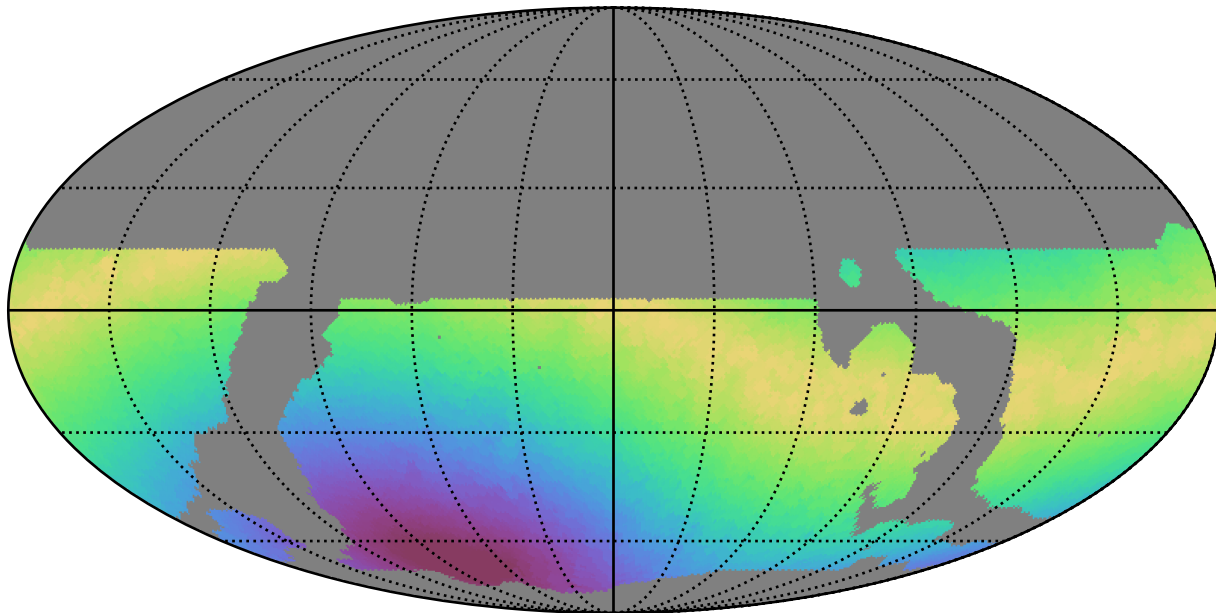
weather_cloudso4v3.4_10yrs WFD i band: Max moonDistance
