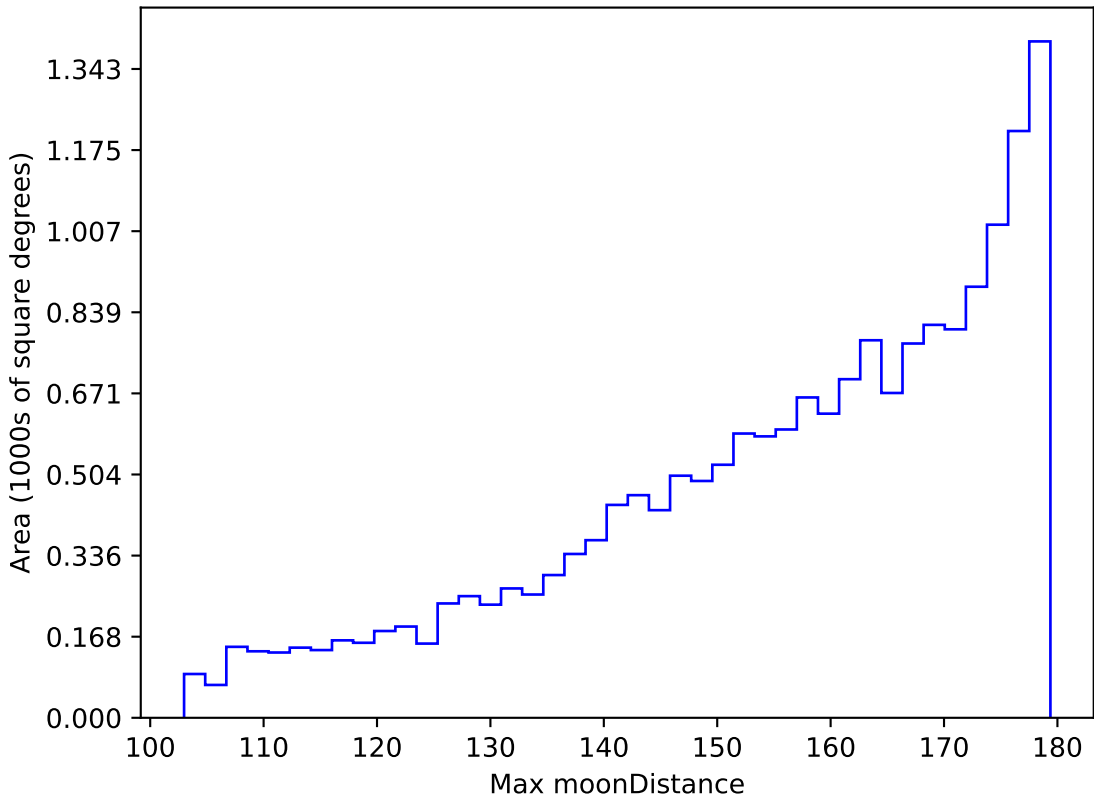
weather_cloudso4v3.4_10yrs WFD i band: Max moonDistance
