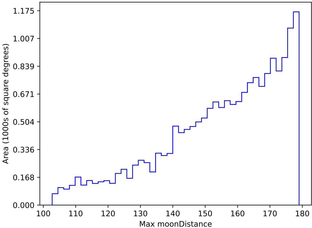
weather_cloudso4v3.4_10yrs WFD g band: Max moonDistance
