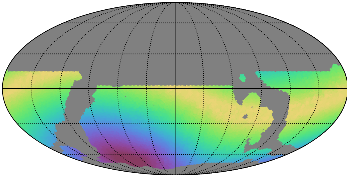
weather_cloudso4v3.4_10yrs WFD all bands: Max moonDistance
