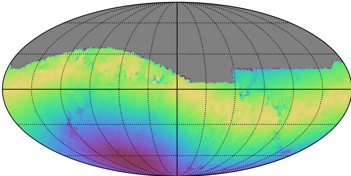
weather_cloudso4v3.4_10yrs All sky z band: Max moonDistance
