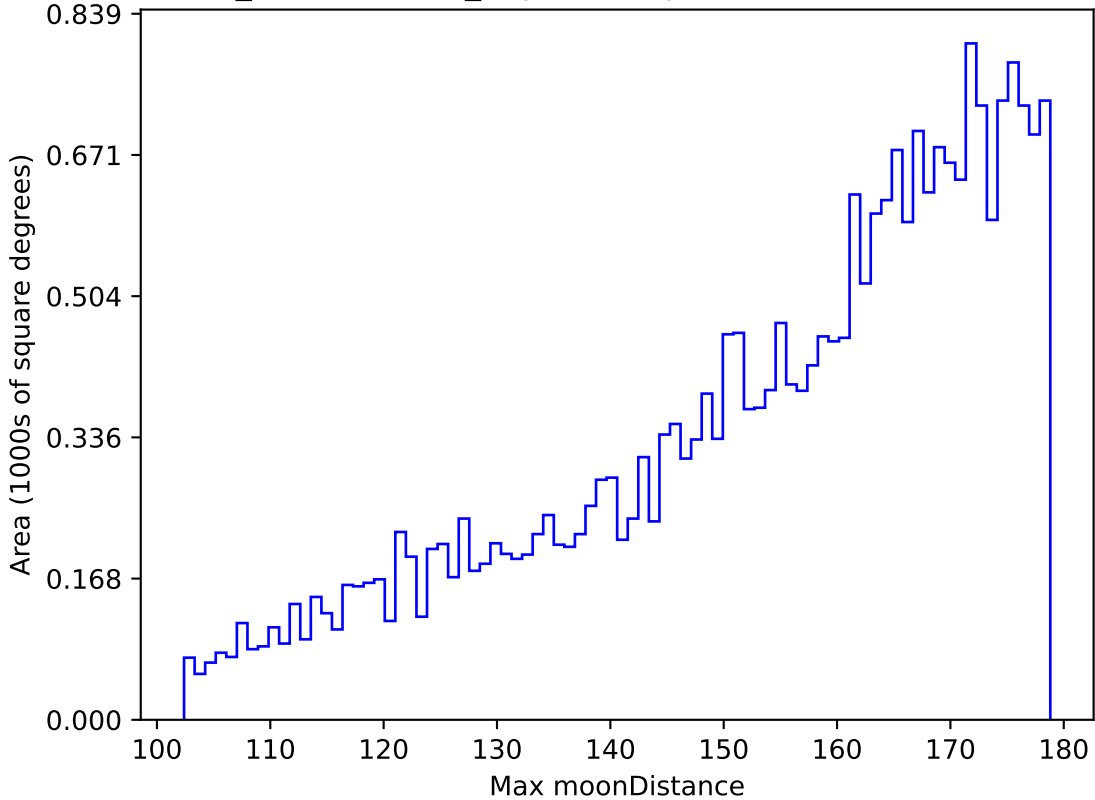
weather_cloudso4v3.4_10yrs All sky z band: Max moonDistance
