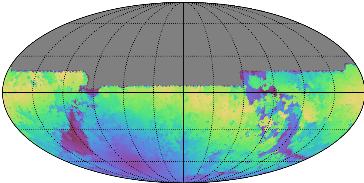
weather_cloudso4v3.4_10yrs All sky y band: Max moonDistance
