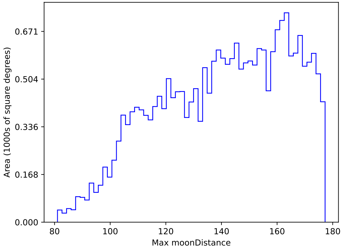
weather_cloudso4v3.4_10yrs All sky y band: Max moonDistance
