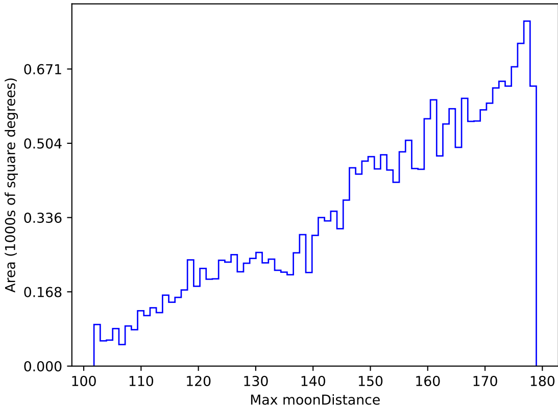
weather_cloudso4v3.4_10yrs All sky u band: Max moonDistance
