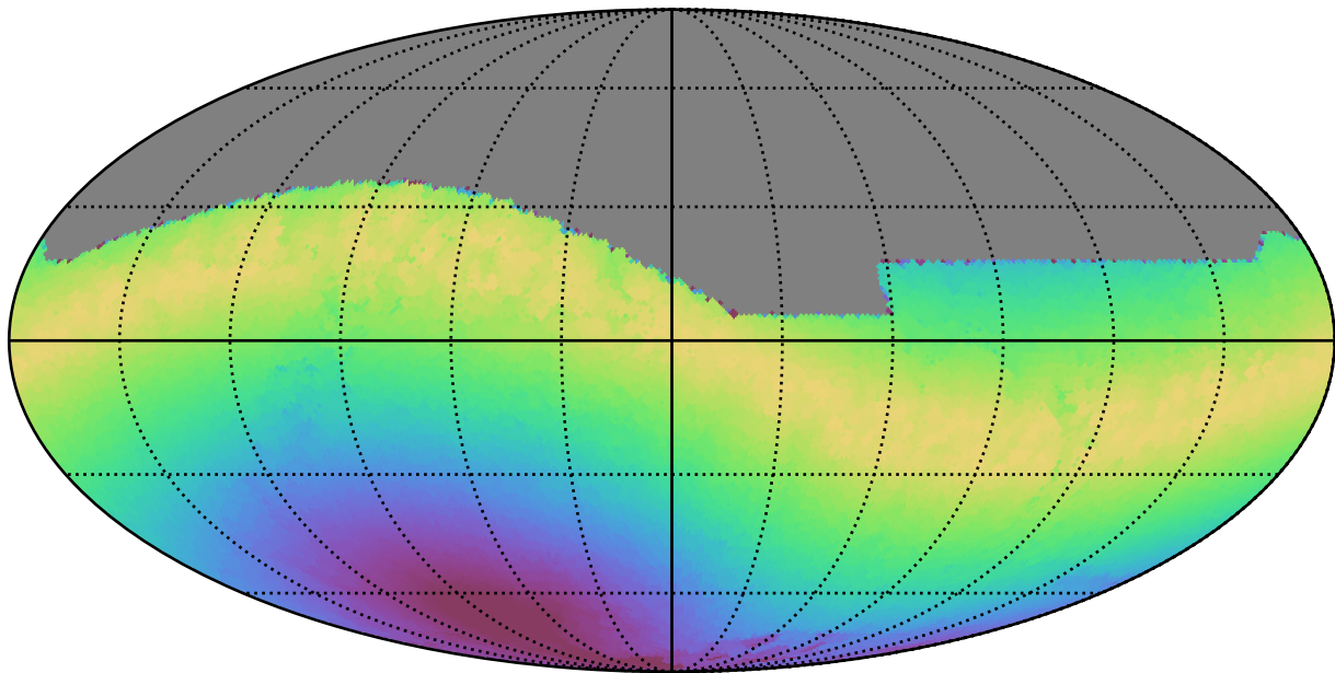
weather_cloudso4v3.4_10yrs All sky r band: Max moonDistance
