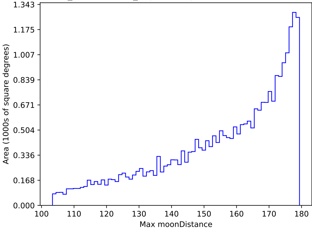
weather_cloudso4v3.4_10yrs All sky r band: Max moonDistance
