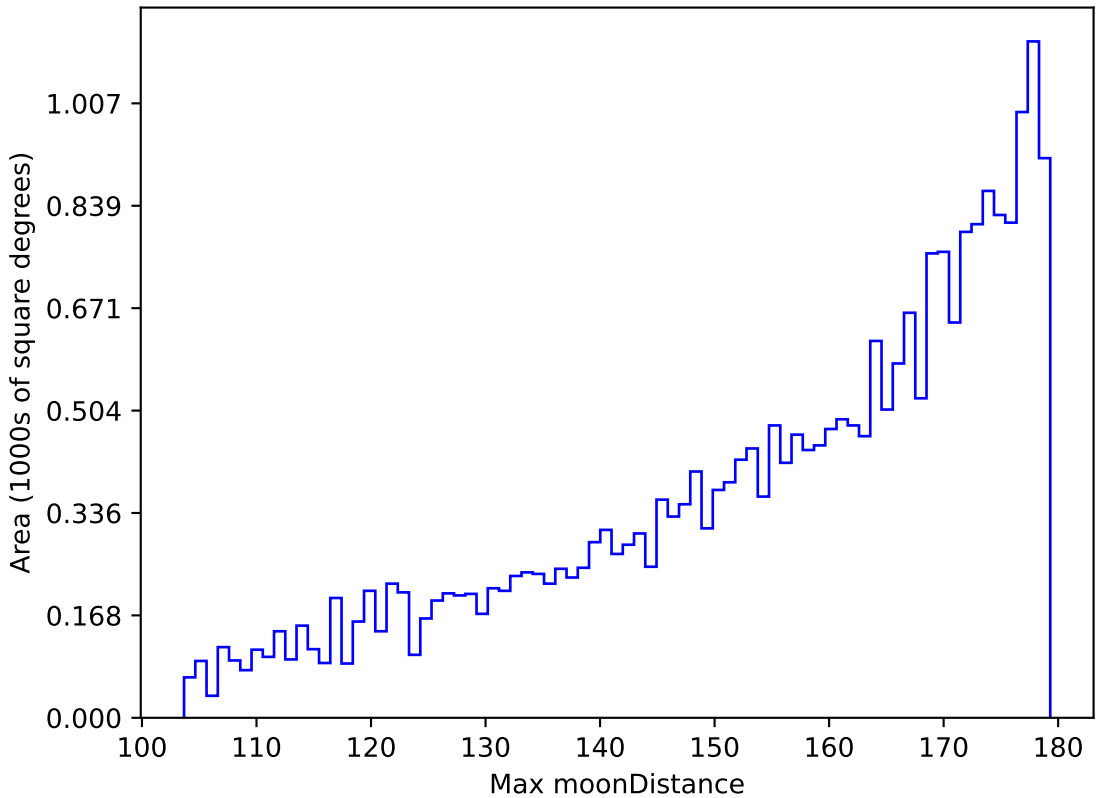
weather_cloudso4v3.4_10yrs All sky i band: Max moonDistance
