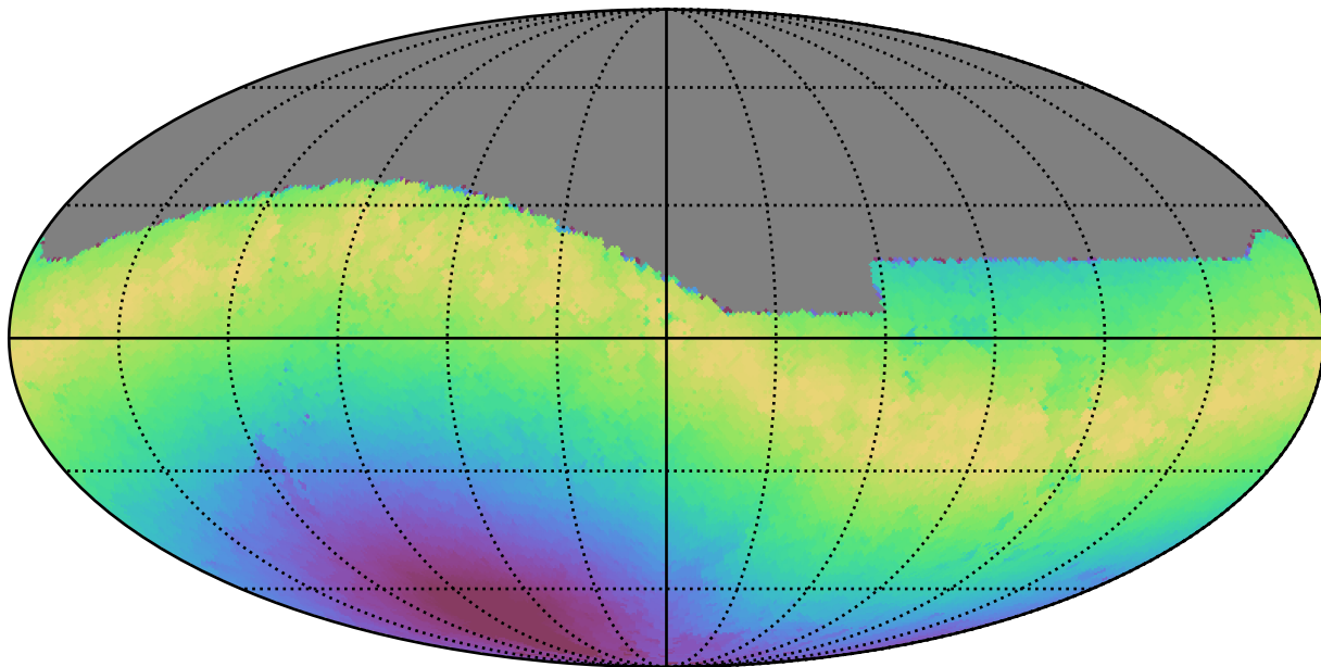
weather_cloudso4v3.4_10yrs All sky g band: Max moonDistance
