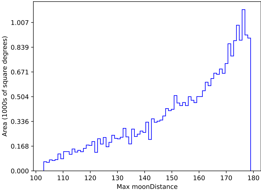
weather_cloudso4v3.4_10yrs All sky g band: Max moonDistance
