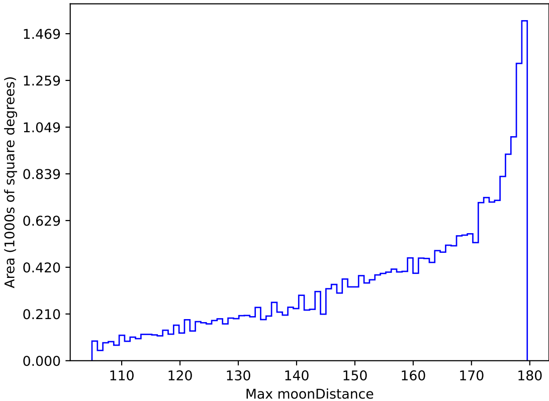
weather_cloudso4v3.4_10yrs All sky all bands: Max moonDistance
