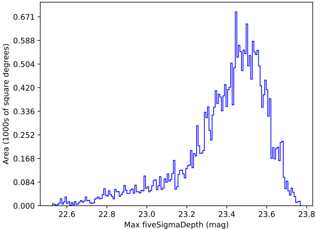
weather_cloudso4v3.4_10yrs Yr 1 z band: Max fiveSigmaDepth
