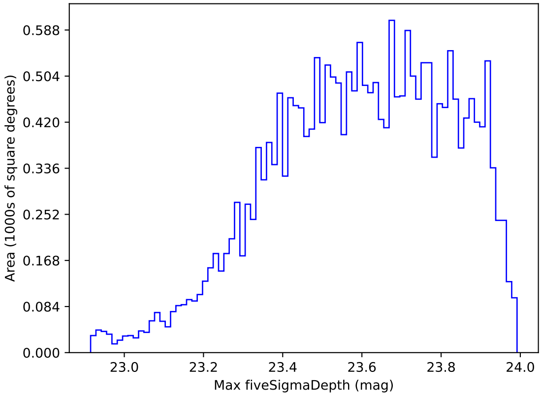
weather_cloudso4v3.4_10yrs Yr 1 u band: Max fiveSigmaDepth
