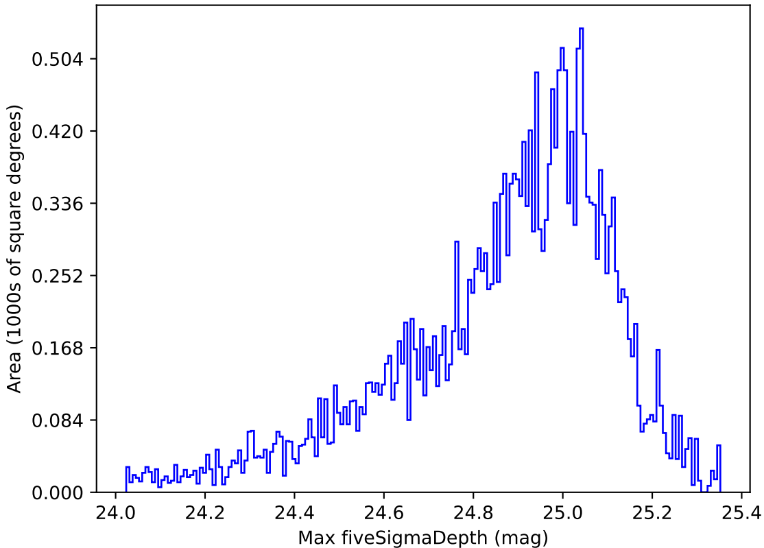
weather_cloudso4v3.4_10yrs Yr 1 g band: Max fiveSigmaDepth
