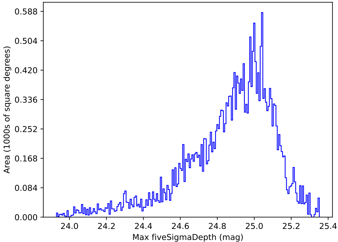
weather_cloudso4v3.4_10yrs Yr 1 all bands: Max fiveSigmaDepth
