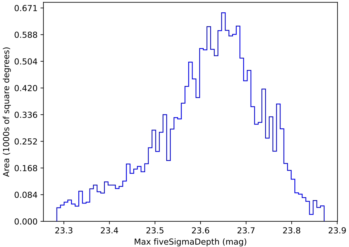
weather_cloudso4v3.4_10yrs WFD z band: Max fiveSigmaDepth
