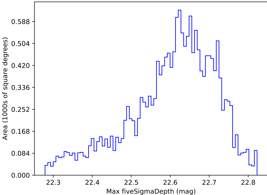
weather_cloudso4v3.4_10yrs WFD y band: Max fiveSigmaDepth
