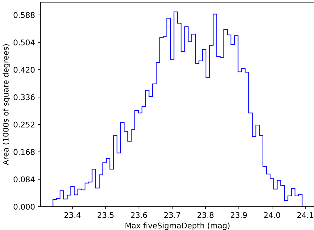
weather_cloudso4v3.4_10yrs WFD u band: Max fiveSigmaDepth
