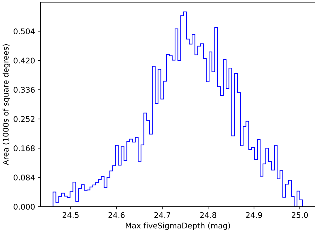
weather_cloudso4v3.4_10yrs WFD r band: Max fiveSigmaDepth
