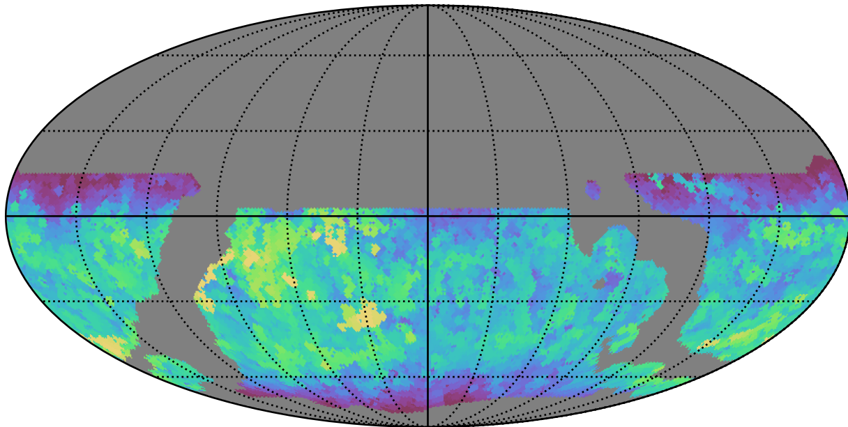
weather_cloudso4v3.4_10yrs WFD i band: Max fiveSigmaDepth
