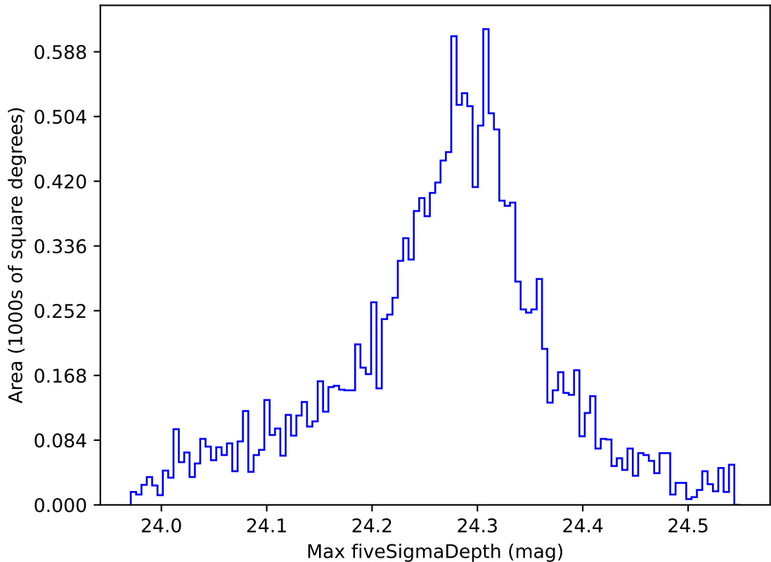
weather_cloudso4v3.4_10yrs WFD i band: Max fiveSigmaDepth
