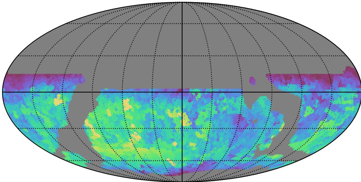
weather_cloudso4v3.4_10yrs WFD g band: Max fiveSigmaDepth
