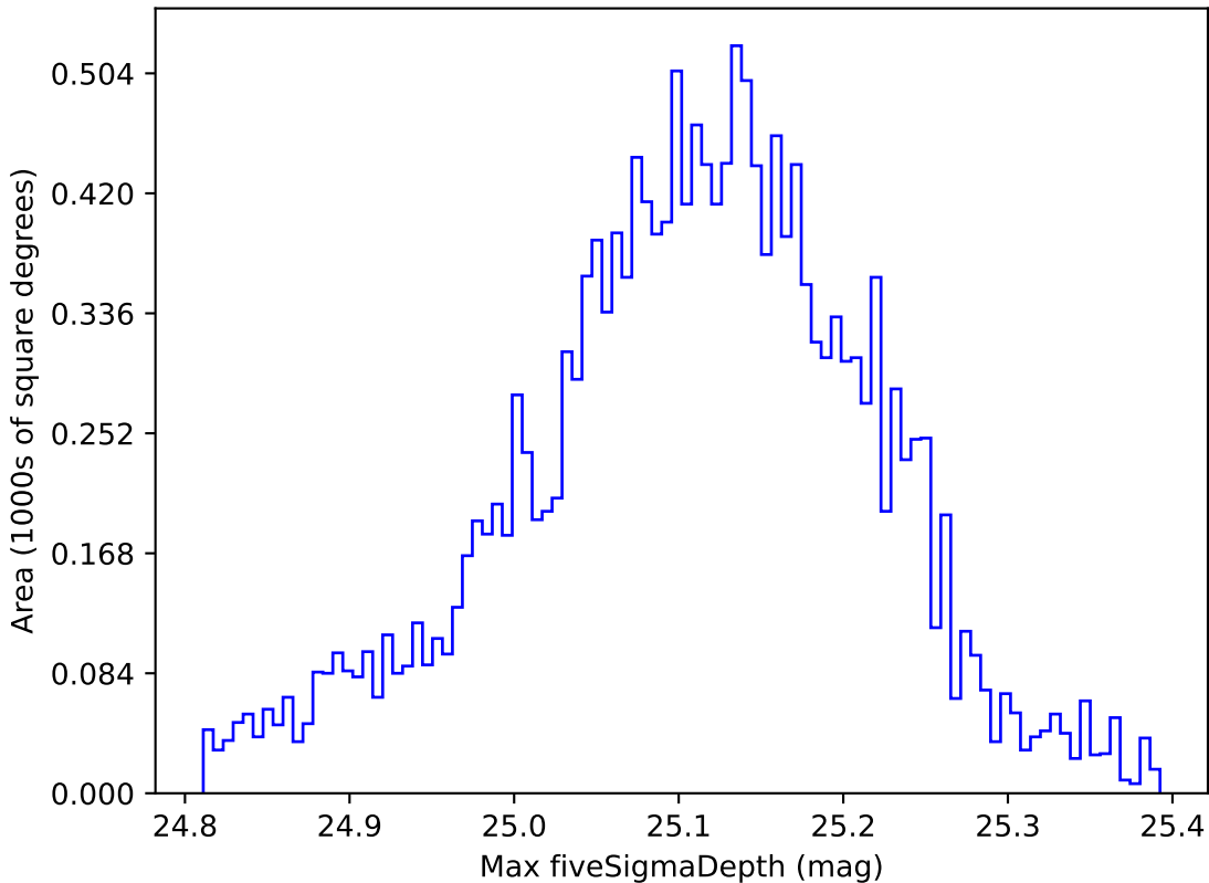
weather_cloudso4v3.4_10yrs WFD g band: Max fiveSigmaDepth
