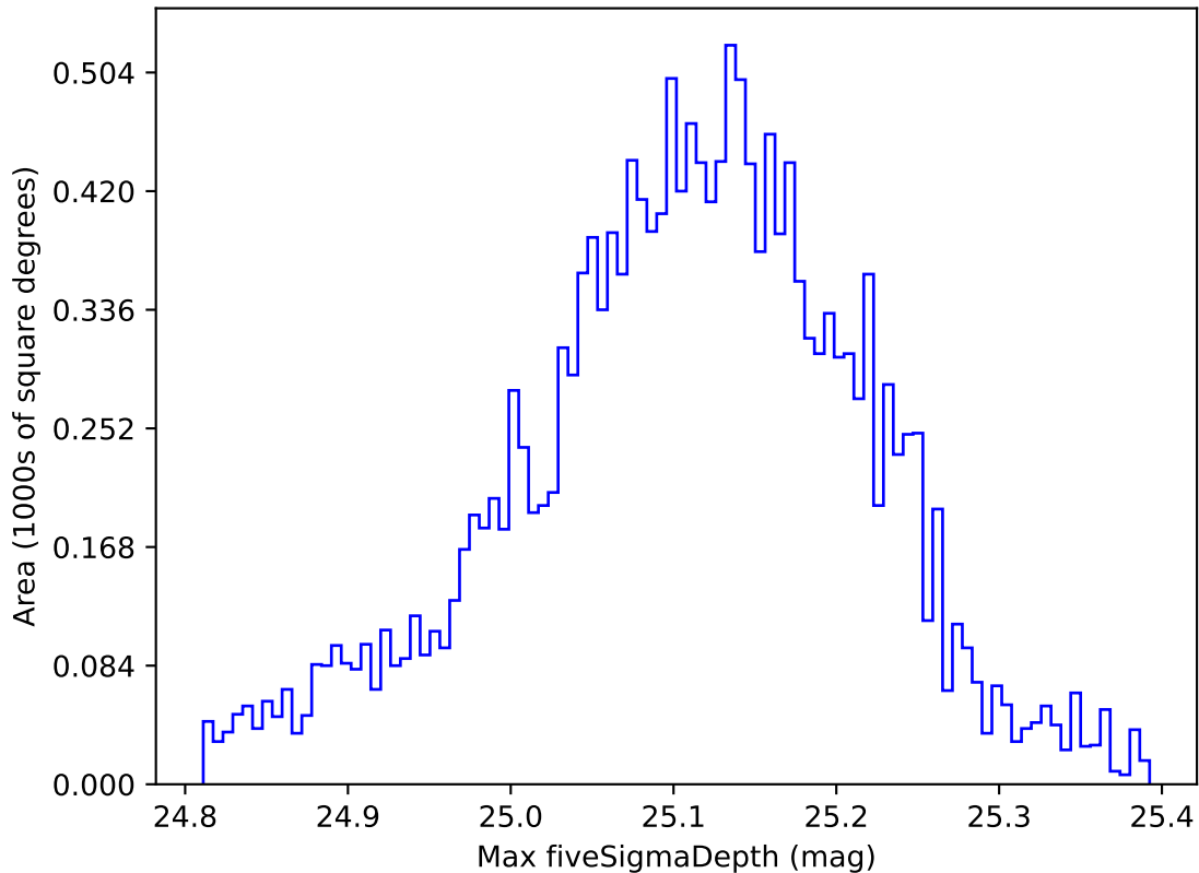
weather_cloudso4v3.4_10yrs WFD all bands: Max fiveSigmaDepth
