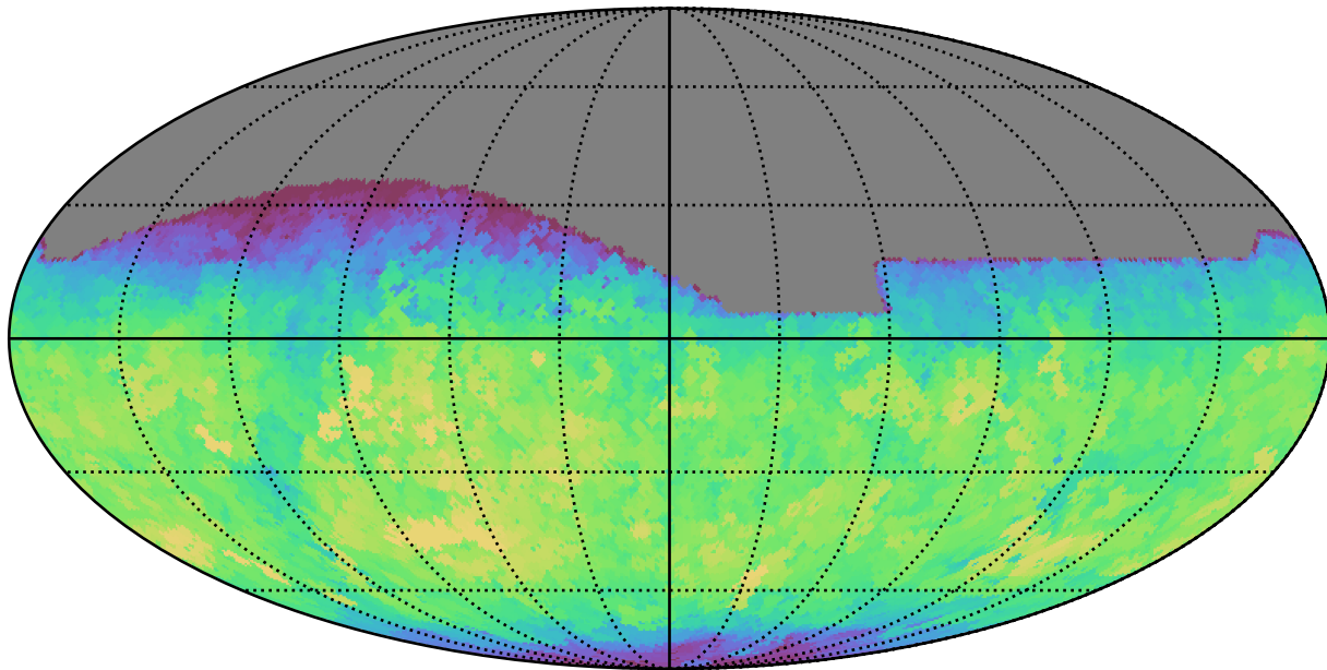
weather_cloudso4v3.4_10yrs All sky z band: Max fiveSigmaDepth
