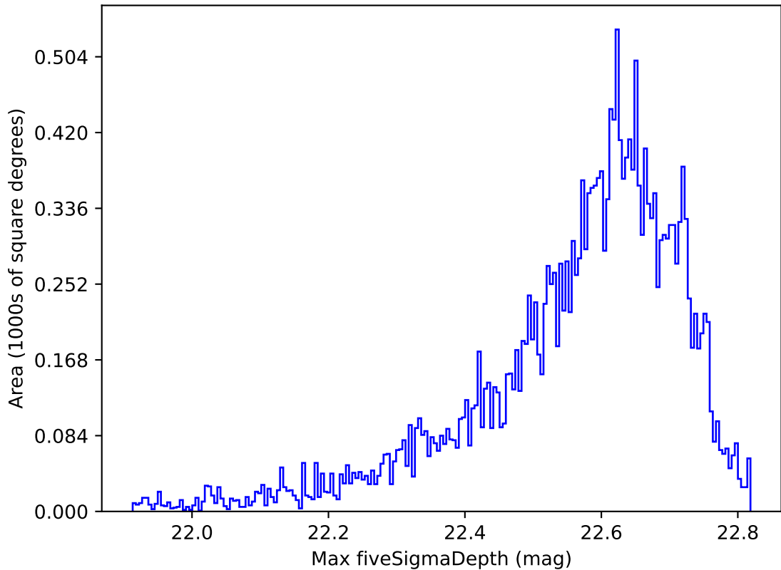
weather_cloudso4v3.4_10yrs All sky y band: Max fiveSigmaDepth
