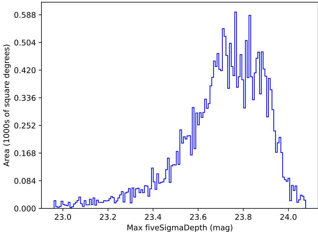
weather_cloudso4v3.4_10yrs All sky u band: Max fiveSigmaDepth
