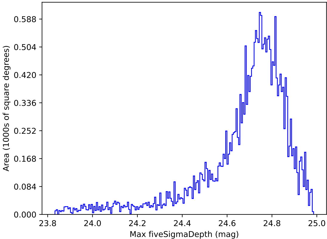
weather_cloudso4v3.4_10yrs All sky r band: Max fiveSigmaDepth
