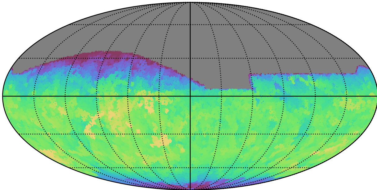
weather_cloudso4v3.4_10yrs All sky i band: Max fiveSigmaDepth
