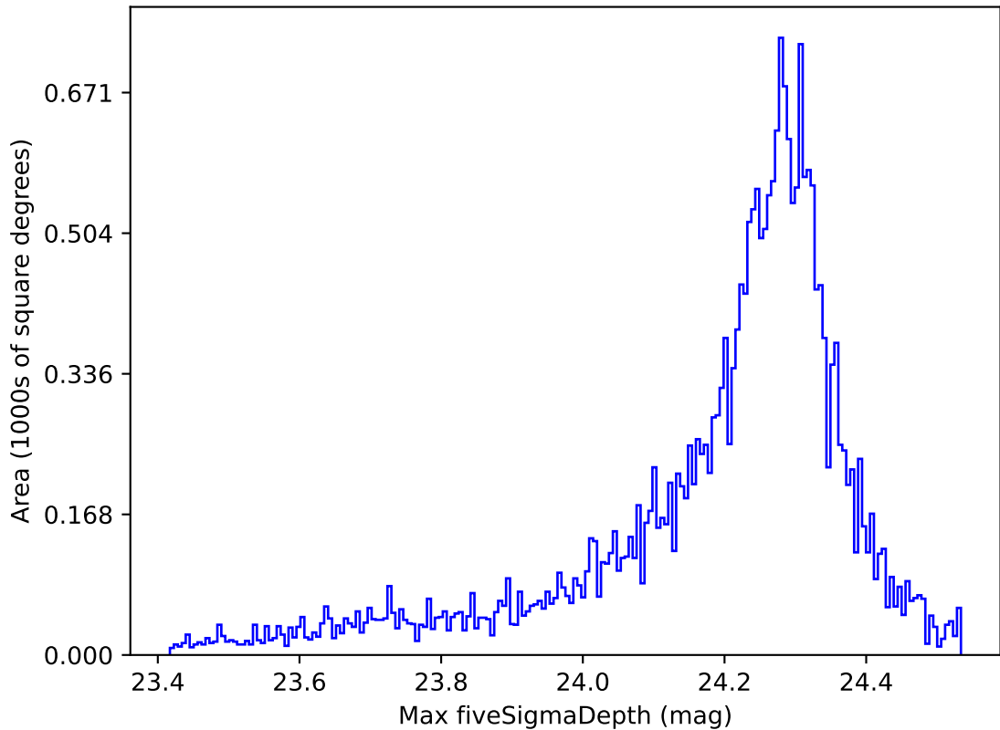
weather_cloudso4v3.4_10yrs All sky i band: Max fiveSigmaDepth
