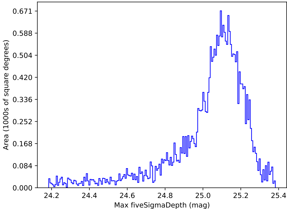
weather_cloudso4v3.4_10yrs All sky g band: Max fiveSigmaDepth
